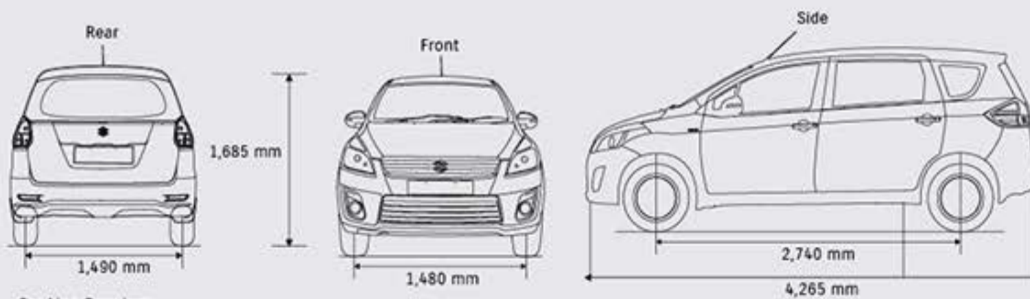
Car Line Drawings
